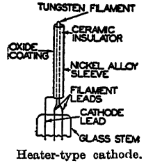
Heater-type cathode.
